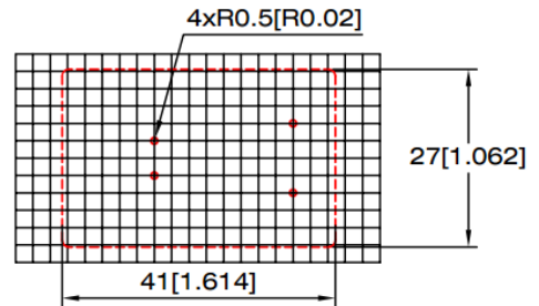
PC Board
